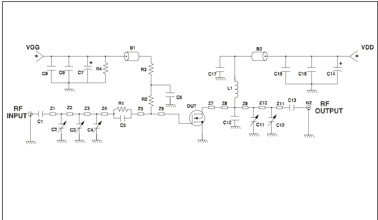
Figure 24. Test circuit schematic
